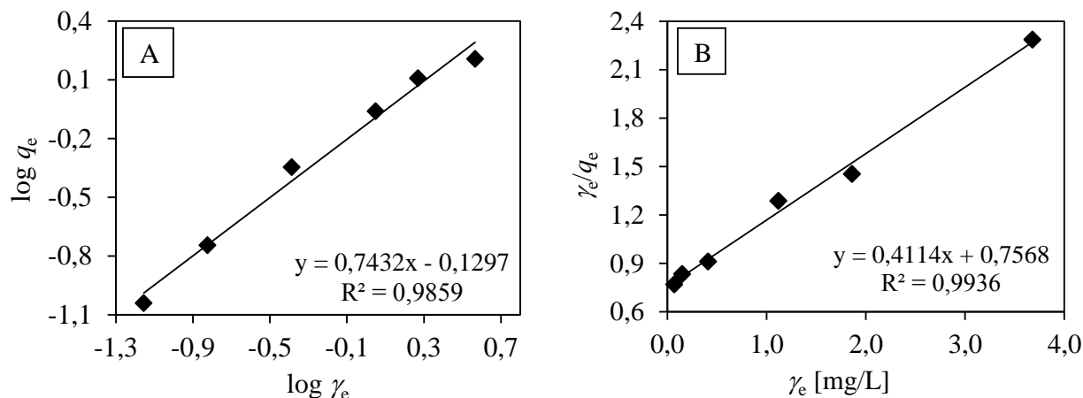
Figure 8. The linearized (A) Freundlich and (B) Langmuir adsorption isotherms for the sorption of ENRO by natural zeolite
