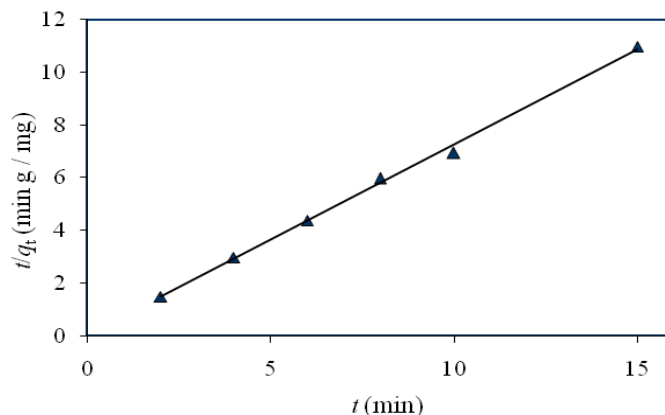
Figure 7. Linearized pseudo-second-order plots for the sorption of ENRO by natural zeolite. Slika 7. Linearizirani graf sorpcije ENRO na prirodni zeolit prema kinetičkom modelu pseudo-drugog reda.
